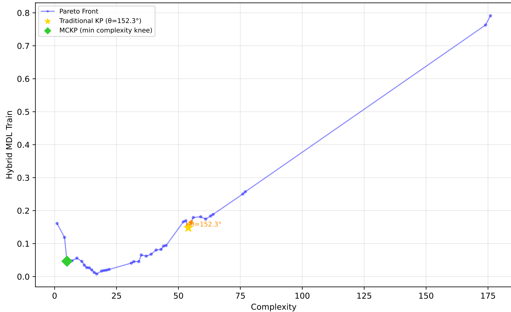
1028_SWD - Run 14 - MVP - Hybrid MDL Train \lambda_1=0.00, \lambda_2=0.00, \lambda_3=0.00 | Difficulty: 1.00 | Method: hmr
