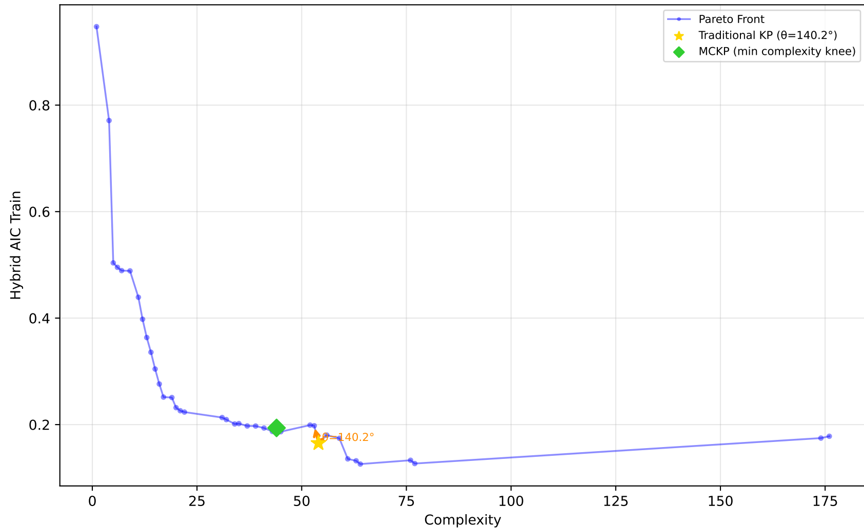
1028_SWD - Run 14 - SVP - Hybrid AIC Train \lambda_1=0.00, \lambda_2=0.60, \lambda_3=0.00 | Difficulty: 1.00 | Method: hmr
