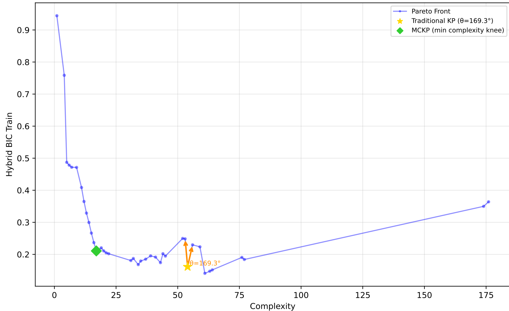
1028_SWD - Run 14 - SVP - Hybrid BIC Train \lambda_1=0.00, \lambda_2=0.60, \lambda_3=0.00 | Difficulty: 1.00 | Method: hmr
