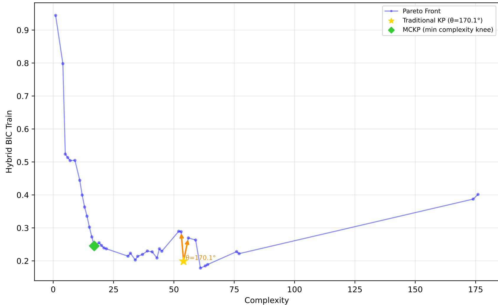
1028_SWD - Run 14 - SVP - Hybrid BIC Train \lambda_1=0.60, \lambda_2=0.00, \lambda_3=0.00 | Difficulty: 1.00 | Method: hmr
