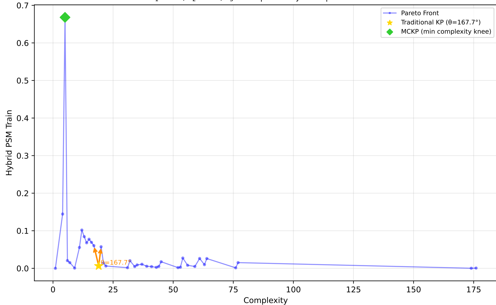
1028_SWD - Run 14 - SVP - Hybrid PSM Train \lambda_1=0.00, \lambda_2=0.60, \lambda_3=0.00 | Difficulty: 1.00 | Method: hmr
