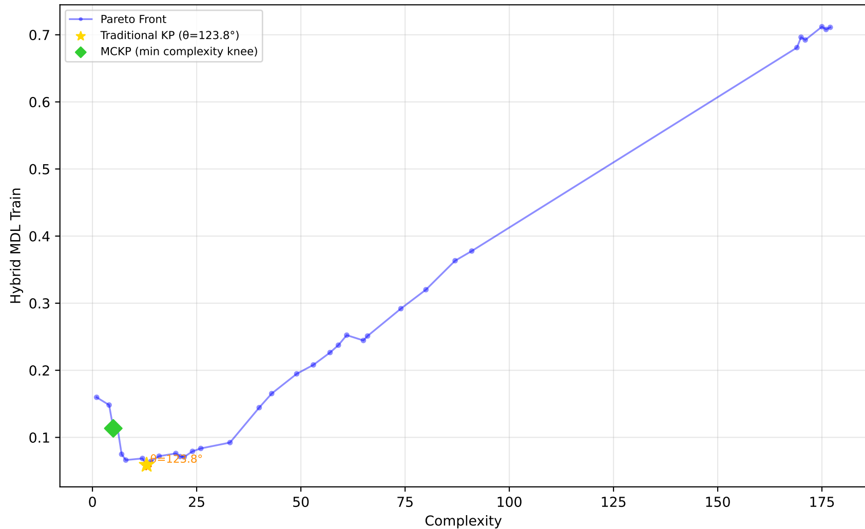
1028_SWD - Run 15 - MVP - Hybrid MDL Train \lambda_1=0.00, \lambda_2=0.00, \lambda_3=0.00 | Difficulty: 1.00 | Method: hmr
