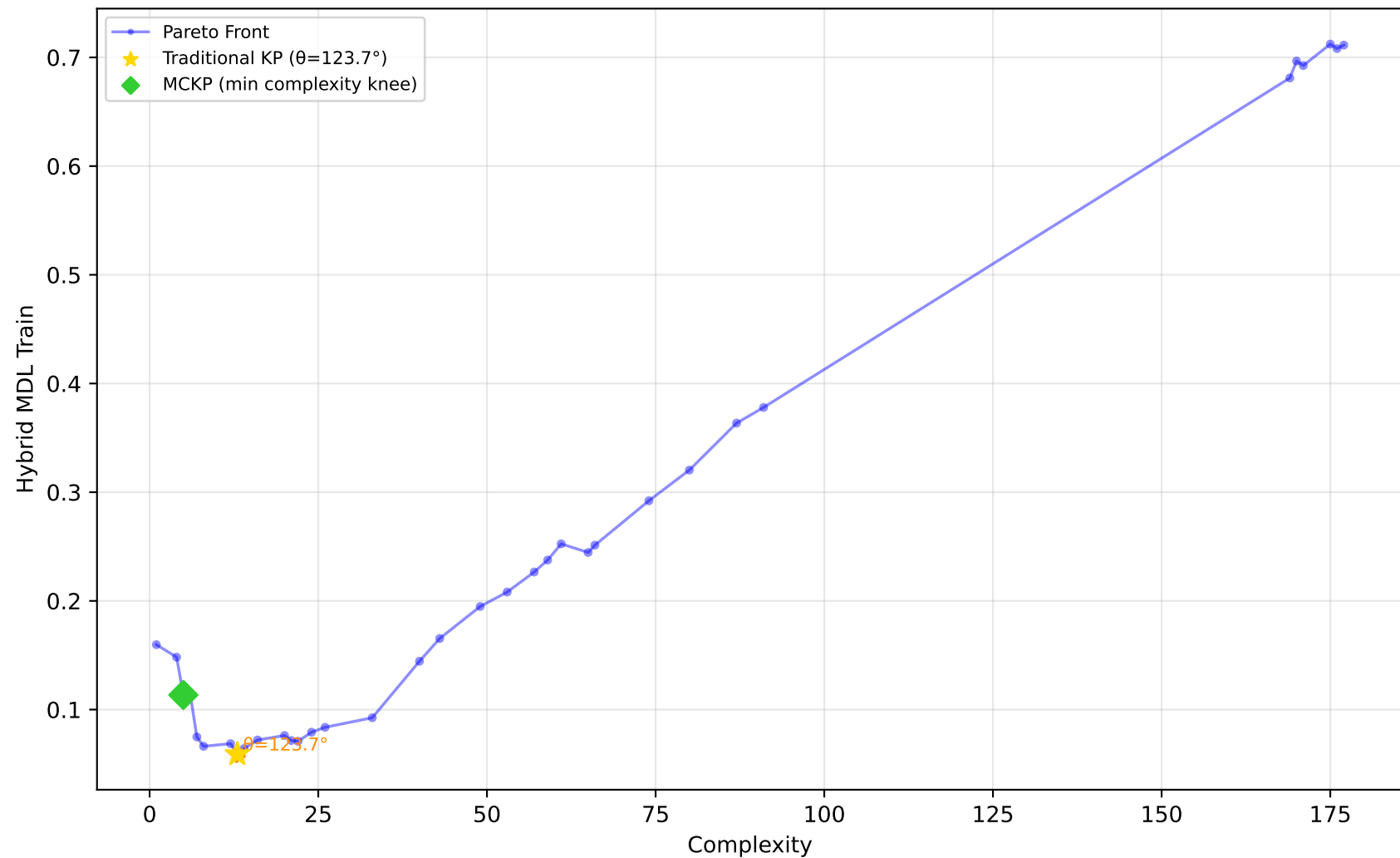
1028_SWD - Run 15 - SVP - Hybrid MDL Train \lambda_1=0.00, \lambda_2=0.60, \lambda_3=0.00 | Difficulty: 1.00 | Method: hmr
