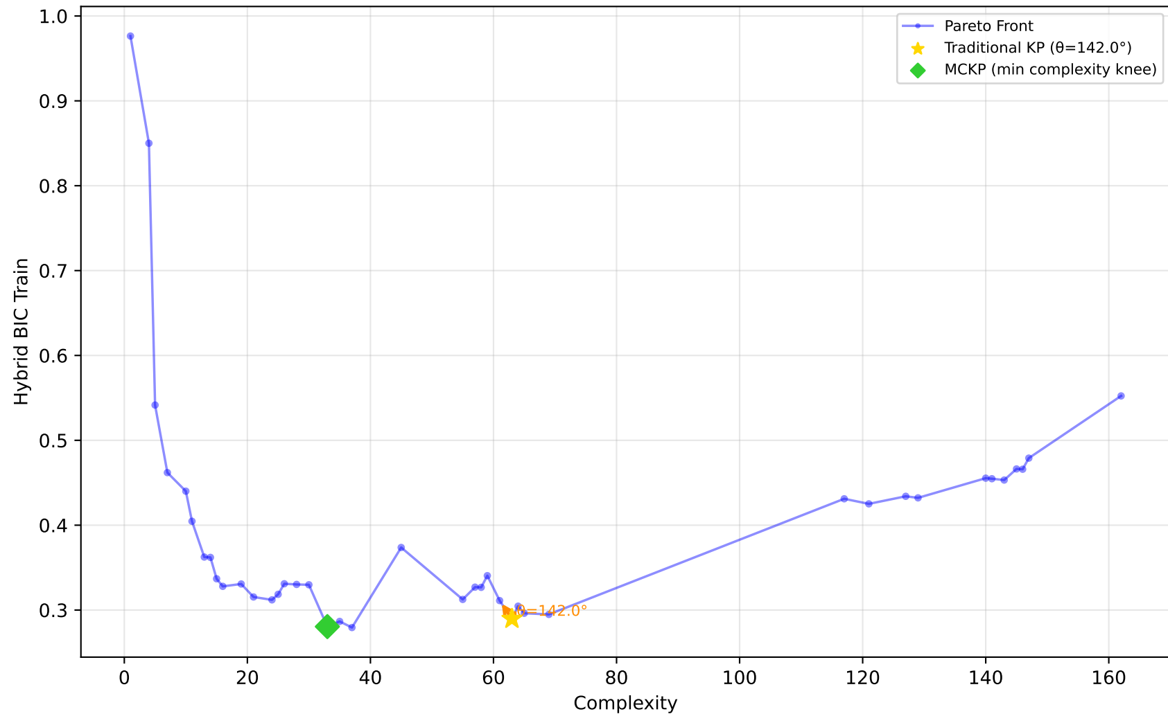
1028_SWD - Run 16 - MVP - Hybrid BIC Train \lambda_1=0.00, \lambda_2=0.00, \lambda_3=0.00 | Difficulty: 1.00 | Method: hmr
