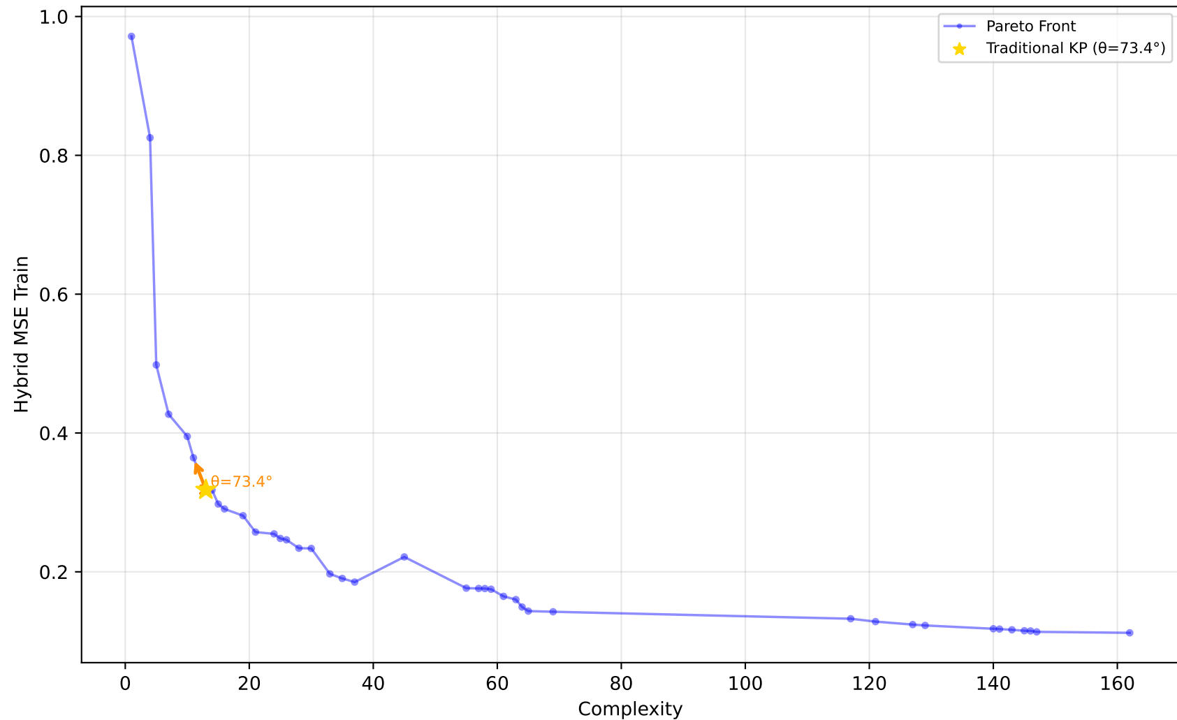
1028_SWD - Run 16 - MVP - Hybrid MSE Train \lambda_1=0.00, \lambda_2=0.00, \lambda_3=0.00 | Difficulty: 1.00 | Method: hmr
