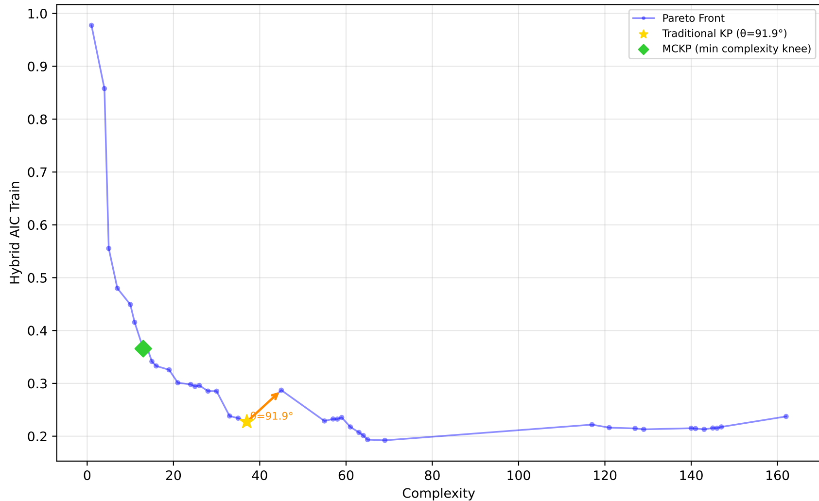
1028_SWD - Run 16 - SVP - Hybrid AIC Train \lambda_1=0.00, \lambda_2=0.60, \lambda_3=0.00 | Difficulty: 1.00 | Method: hmr
