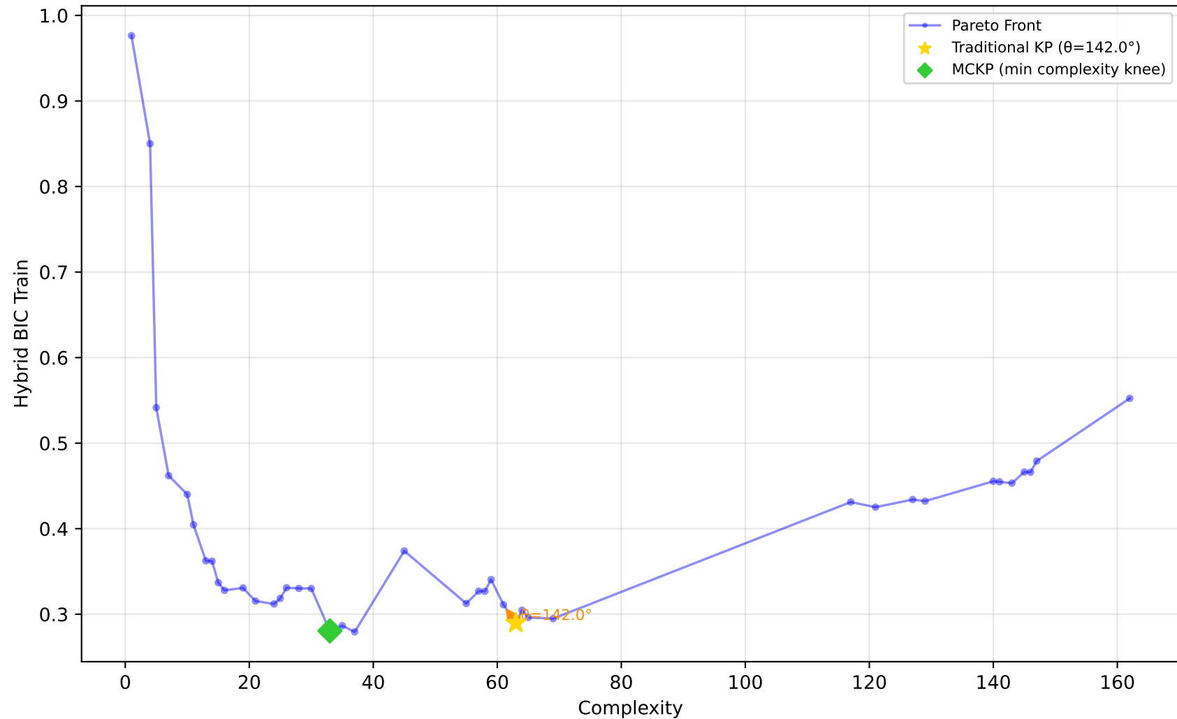
1028_SWD - Run 16 - SVP - Hybrid BIC Train \lambda_1=0.00, \lambda_2=0.60, \lambda_3=0.00 | Difficulty: 1.00 | Method: hmr
