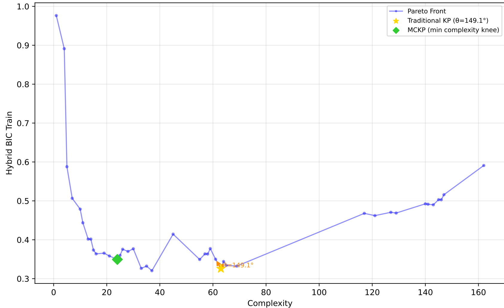
1028_SWD - Run 16 - SVP - Hybrid BIC Train \lambda_1=0.60, \lambda_2=0.00, \lambda_3=0.00 | Difficulty: 1.00 | Method: hmr
