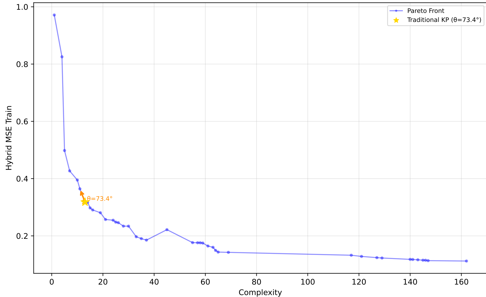
1028_SWD - Run 16 - SVP - Hybrid MSE Train \lambda_1=0.00, \lambda_2=0.60, \lambda_3=0.00 | Difficulty: 1.00 | Method: hmr
