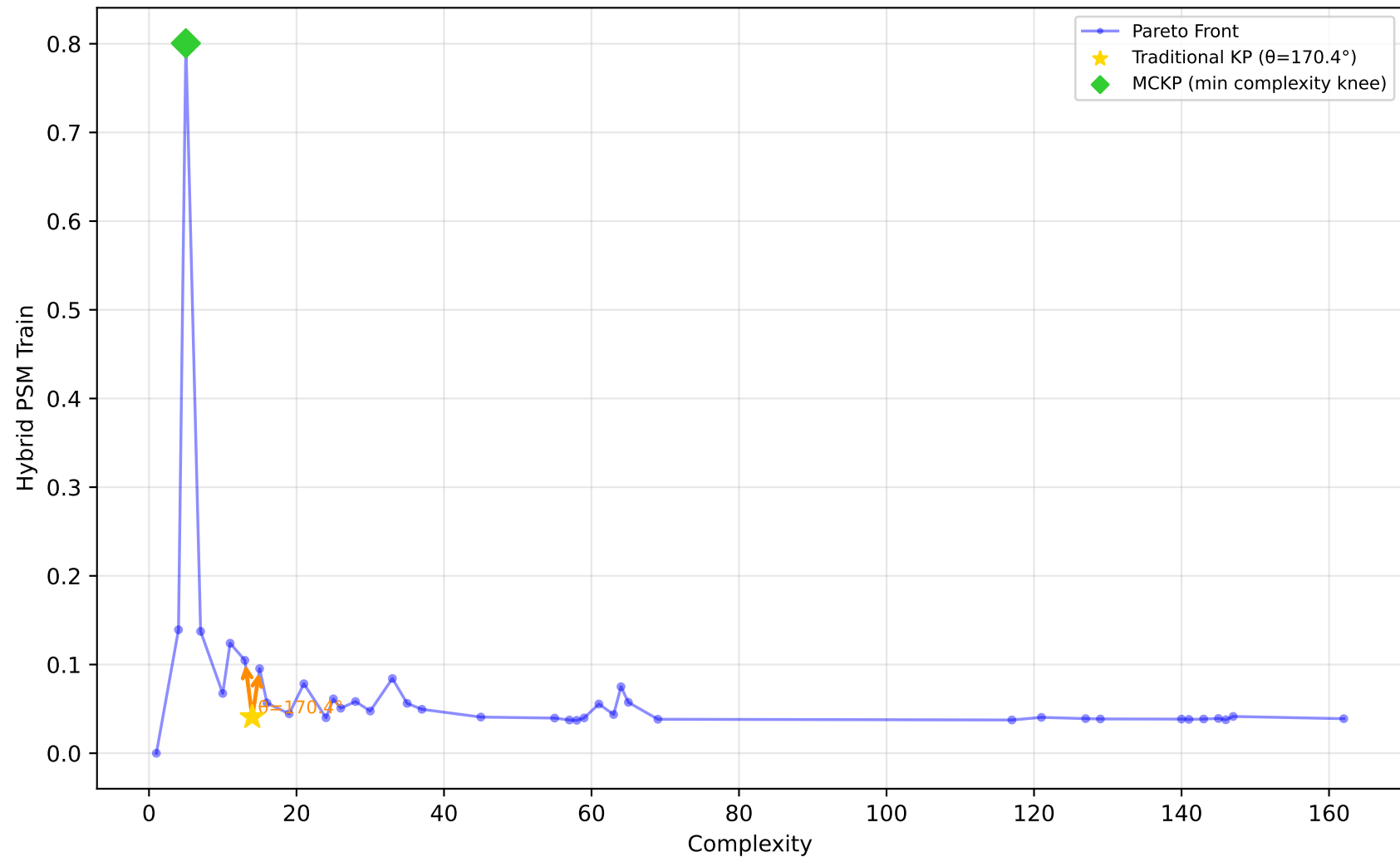
1028_SW D - Run 16 - SVP - Hybrid PSM Train \lambda_1=0.60, \lambda_2=0.00, \lambda_3=0.00 | Difficulty: 1.00 | Method: hmr
