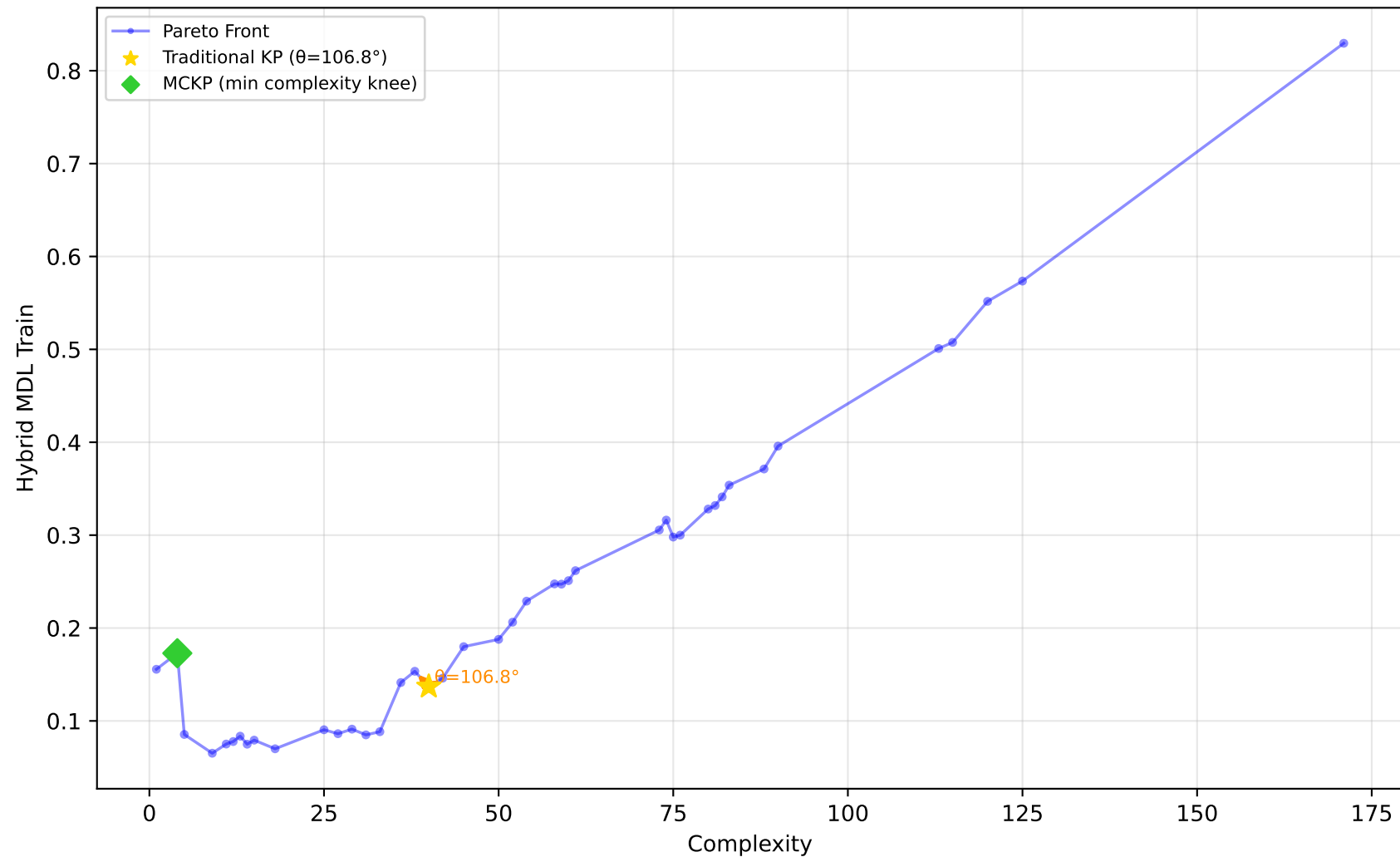
1028_SWD - Run 17 - MVP - Hybrid MDL Train \lambda_1=0.60, \lambda_2=0.00, \lambda_3=0.00 | Difficulty: 1.00 | Method: hmr
