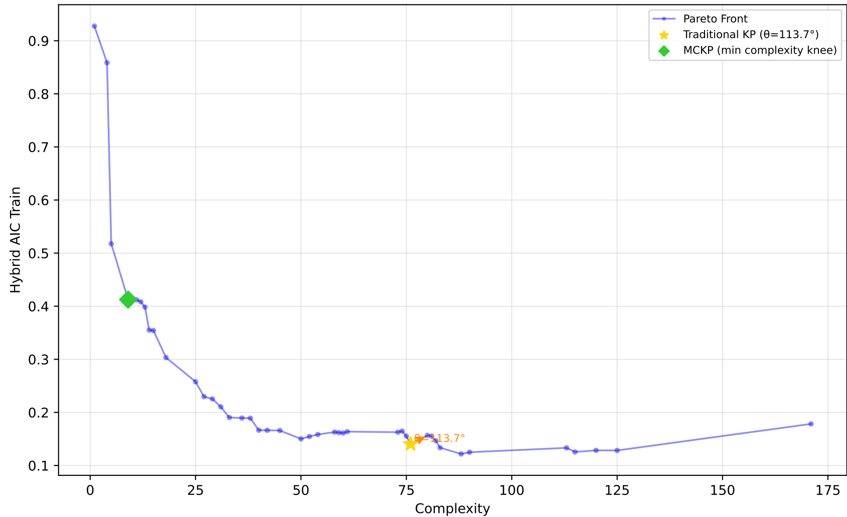
1028_SWD - Run 17 - SVP - Hybrid AIC Train \lambda_1=0.60, \lambda_2=0.00, \lambda_3=0.00 | Difficulty: 1.00 | Method: hmr
