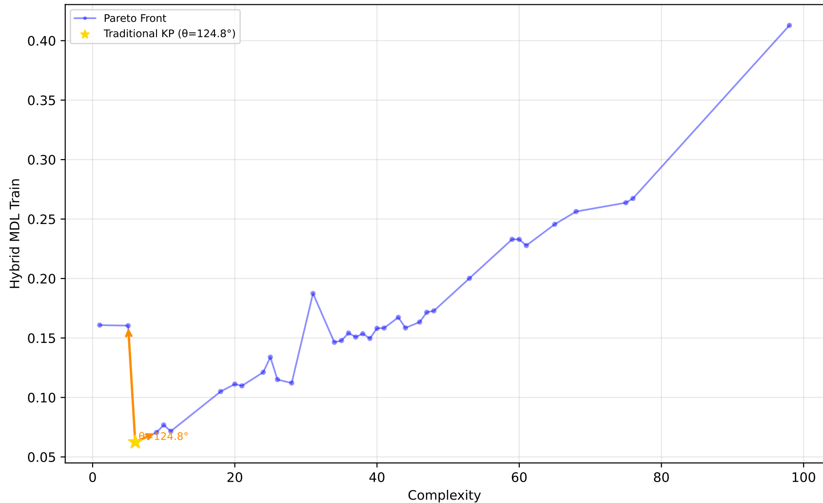
1028_SWD - Run 18 - MVP - Hybrid MDL Train \lambda_1=0.00, \lambda_2=0.00, \lambda_3=0.00 | Difficulty: 1.00 | Method: hmr
