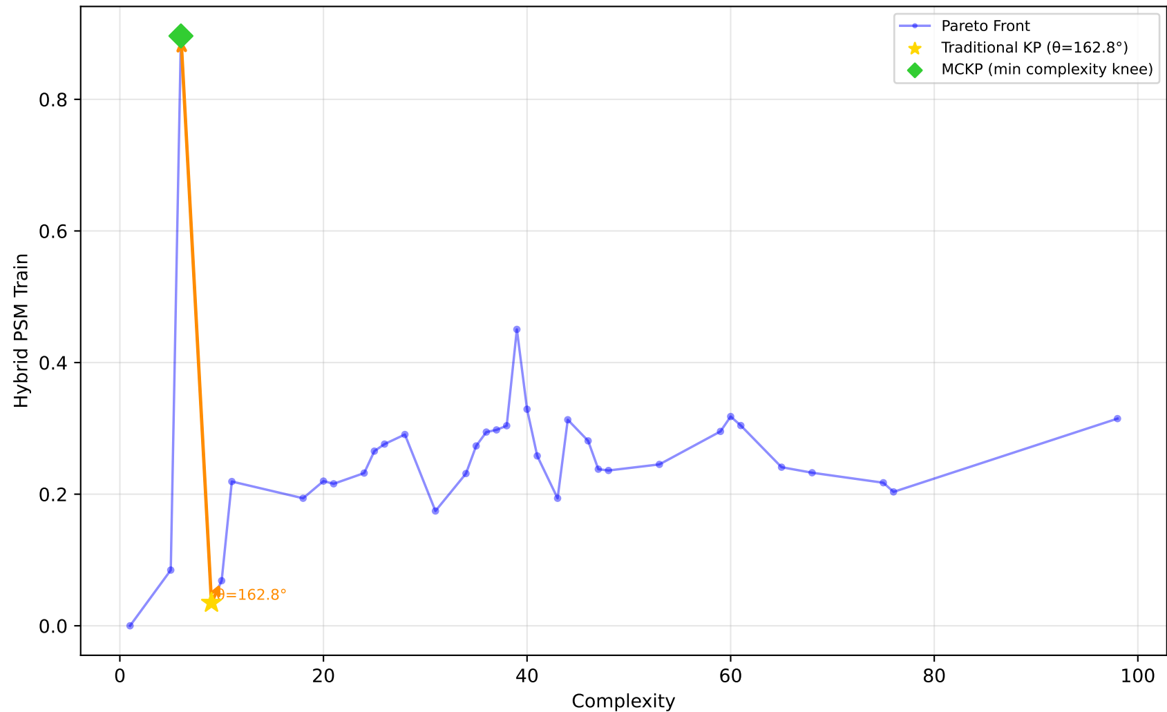
1028_SWD - Run 18 - MVP - Hybrid PSM Train \lambda_1=0.60, \lambda_2=0.00, \lambda_3=0.00 | Difficulty: 1.00 | Method: hmr
