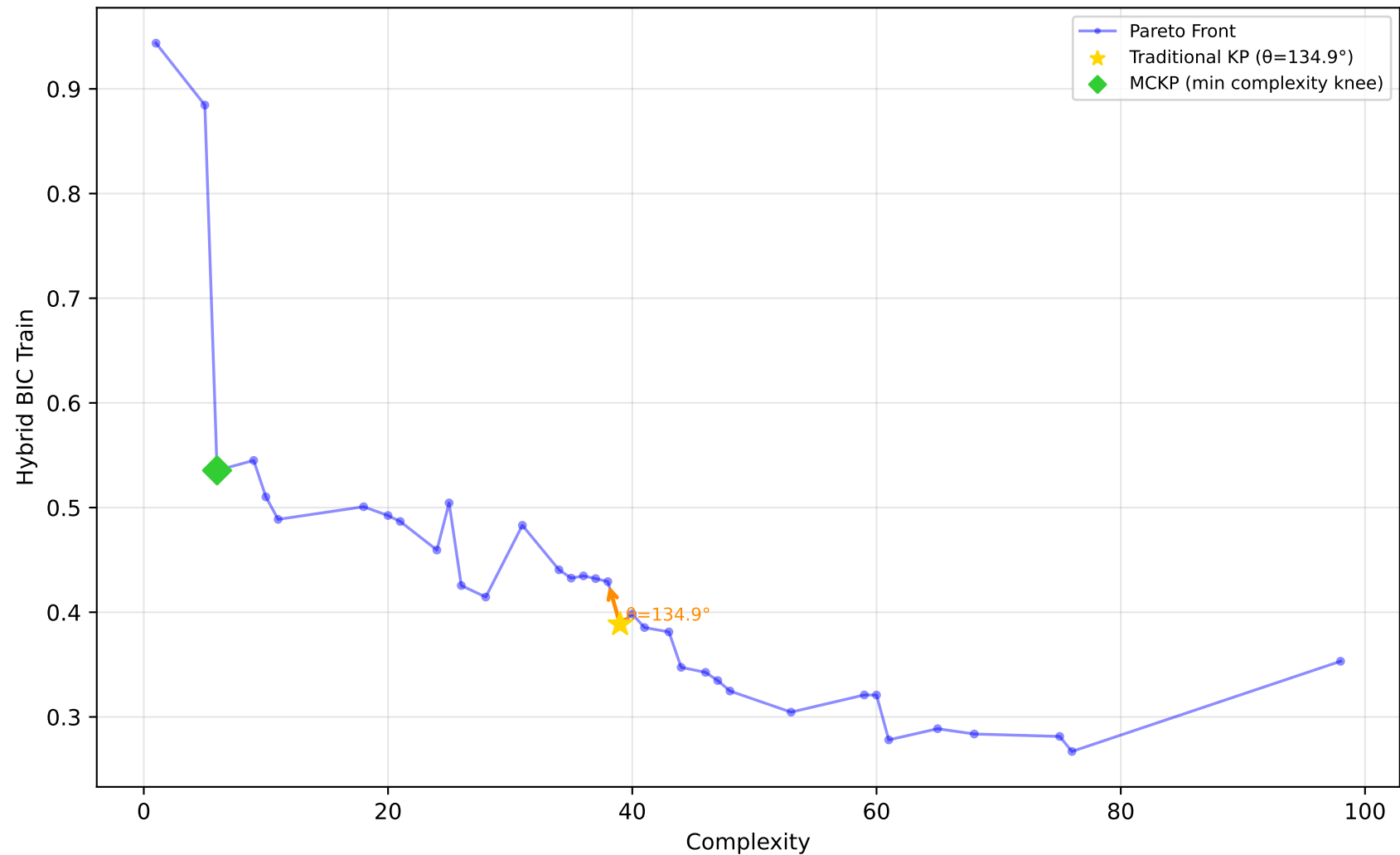
1028_SWD - Run 18 - SVP - Hybrid BIC Train \lambda_1=0.00, \lambda_2=0.60, \lambda_3=0.00 | Difficulty: 1.00 | Method: hmr
