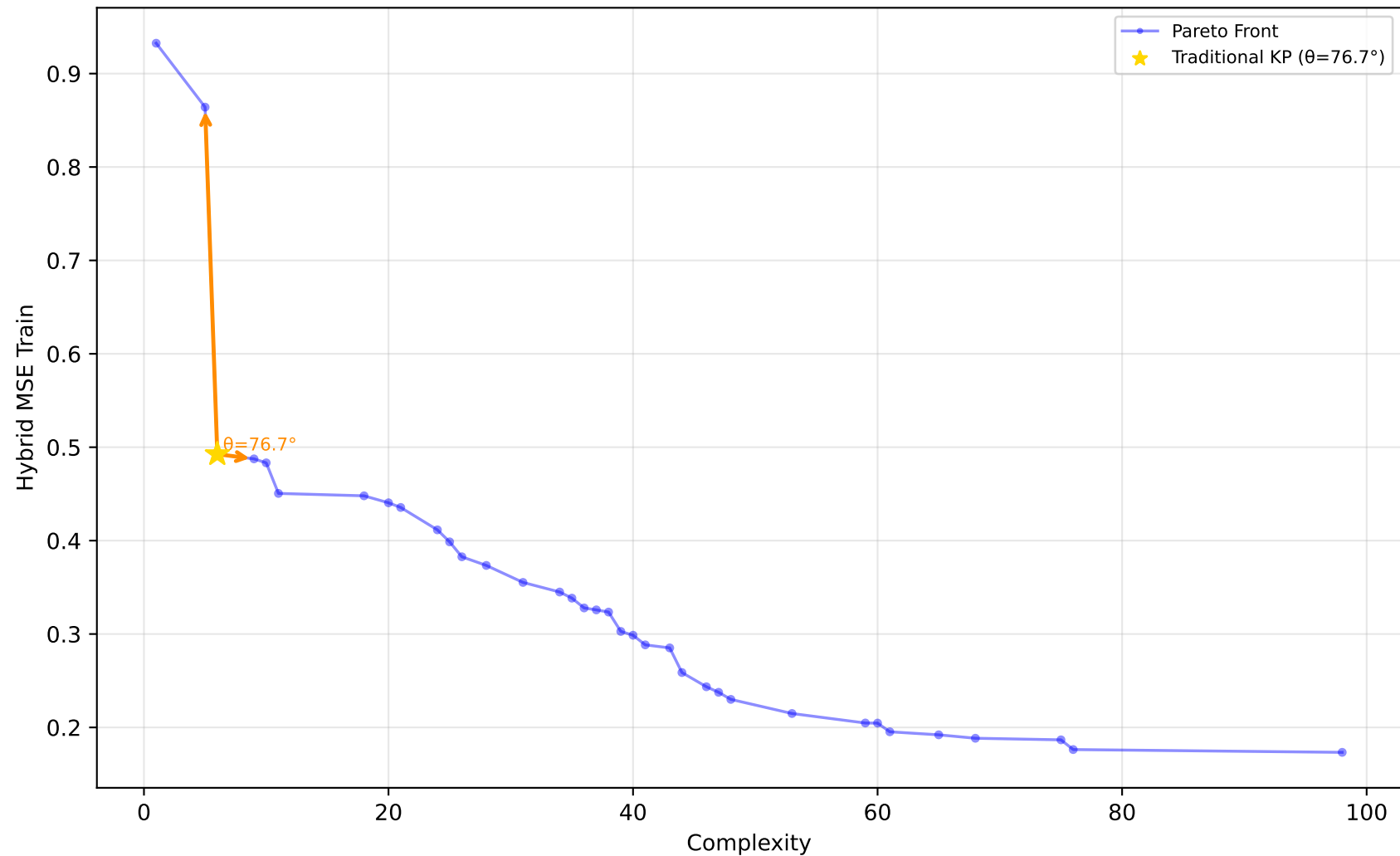
1028_SWD - Run 18 - SVP - Hybrid MSE Train \lambda_1=0.00, \lambda_2=0.60, \lambda_3=0.00 | Difficulty: 1.00 | Method: hmr
