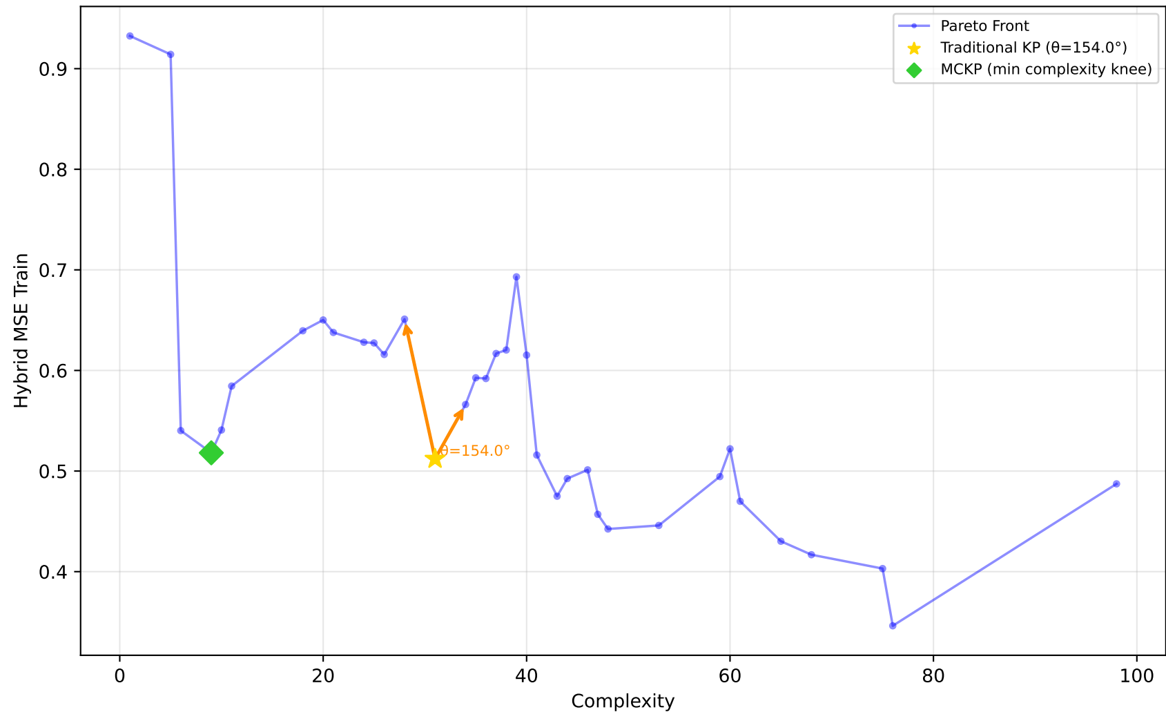
1028_SWD - Run 18 - SVP - Hybrid MSE Train \lambda_1=0.60, \lambda_2=0.00, \lambda_3=0.00 | Difficulty: 1.00 | Method: hmr
