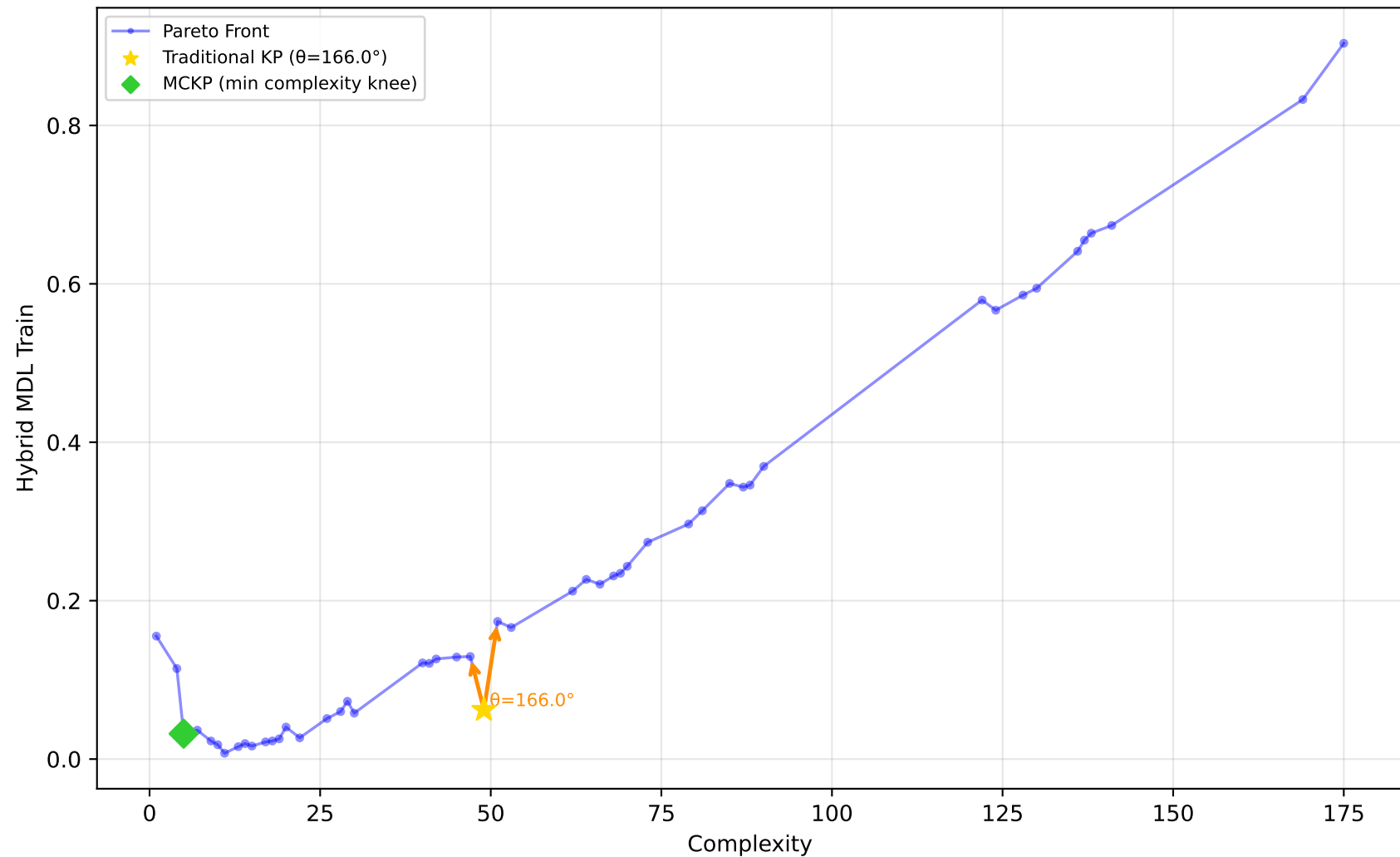
1028_SWD - Run 19 - MVP - Hybrid MDL Train \lambda_1=0.00, \lambda_2=0.00, \lambda_3=0.00 | Difficulty: 1.00 | Method: hmr
