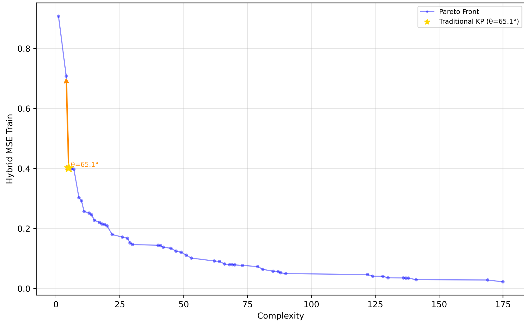
1028_SWD - Run 19 - MVP - Hybrid MSE Train \lambda_1=0.00, \lambda_2=0.00, \lambda_3=0.00 | Difficulty: 1.00 | Method: hmr
