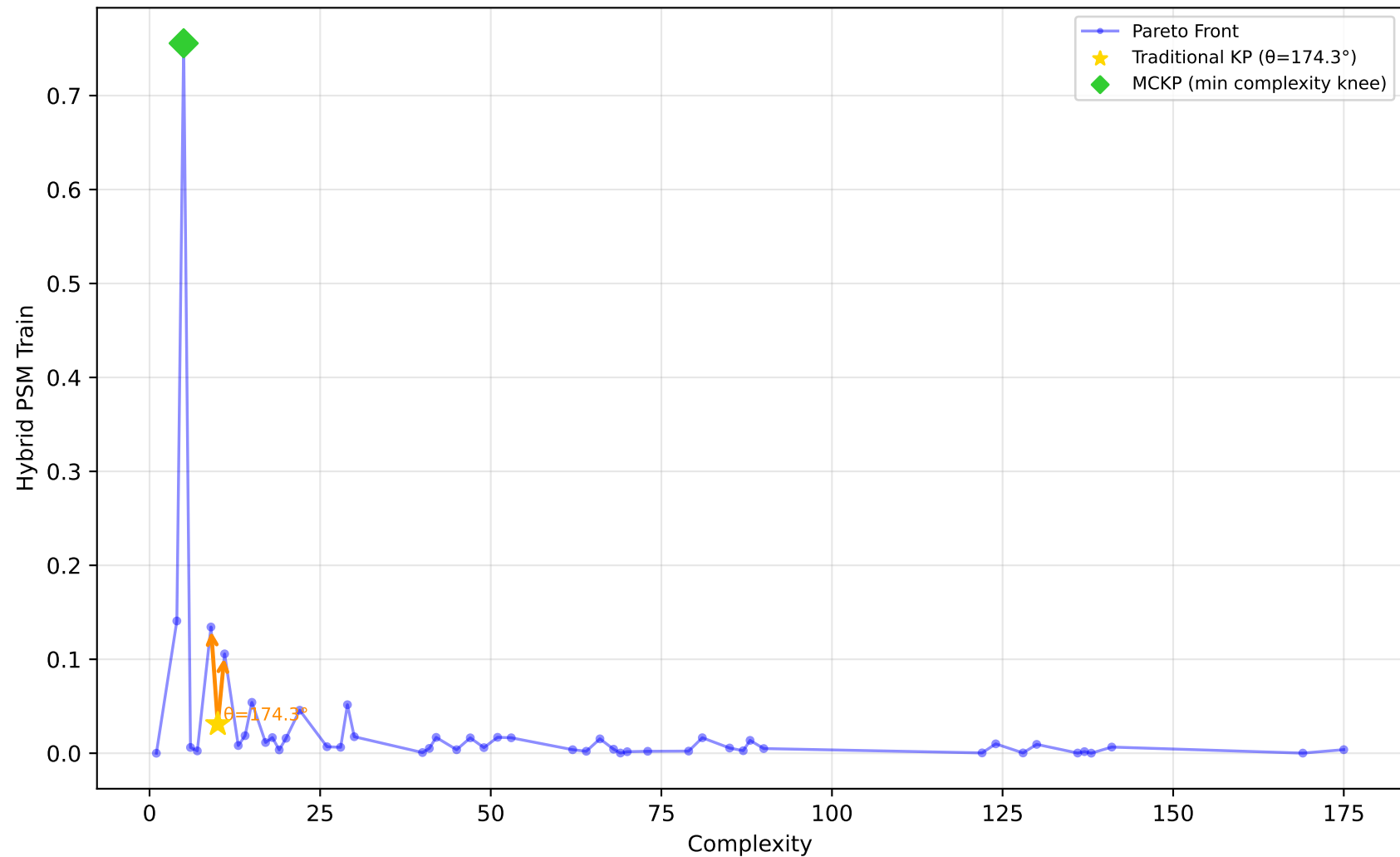
1028_SWD - Run 19 - MVP - Hybrid PSM Train \lambda_1=0.00, \lambda_2=0.00, \lambda_3=0.00 | Difficulty: 1.00 | Method: hmr
