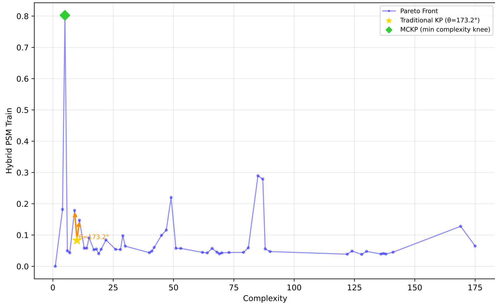
1028_SWD - Run 19 - MVP - Hybrid PSM Train \lambda_1=0.60, \lambda_2=0.00, \lambda_3=0.00 | Difficulty: 1.00 | Method: hmr
