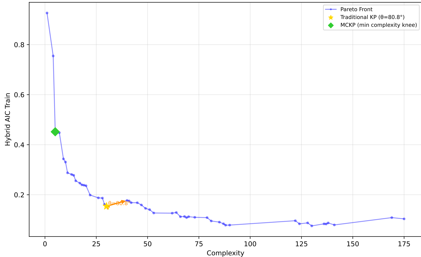
1028_SWD - Run 19 - SVP - Hybrid AIC Train \lambda_1=0.00, \lambda_2=0.60, \lambda_3=0.00 | Difficulty: 1.00 | Method: hmr
