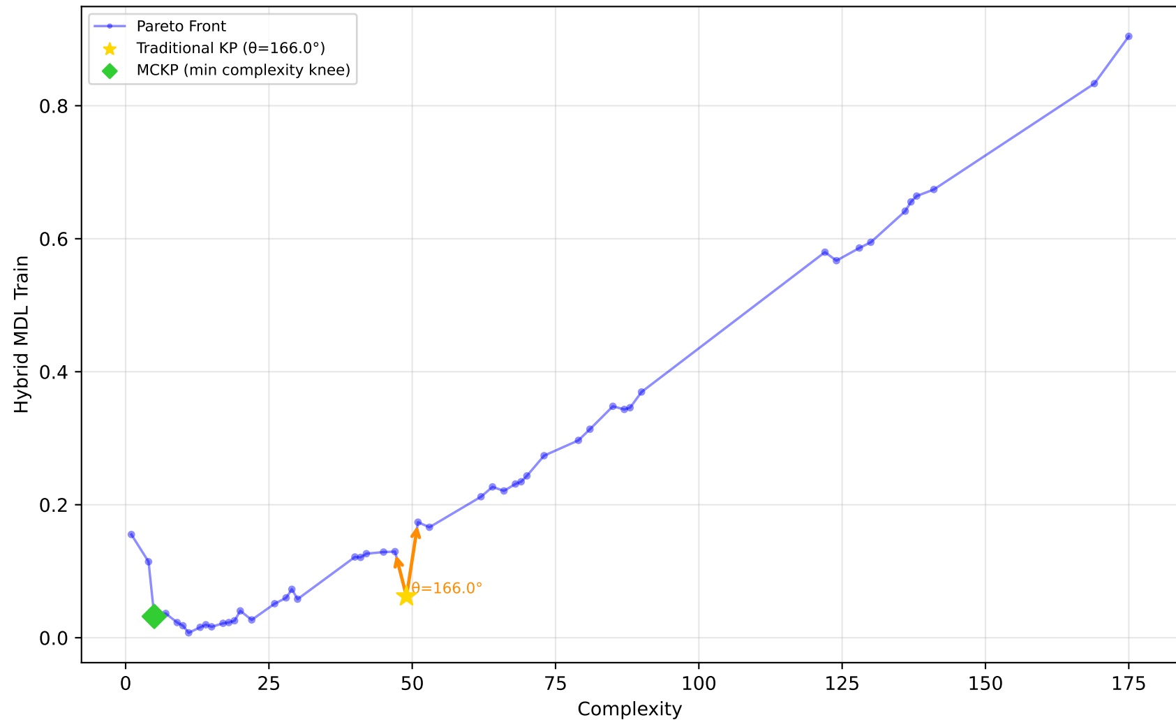
1028_SWD - Run 19 - SVP - Hybrid MDL Train \lambda_1=0.00, \lambda_2=0.60, \lambda_3=0.00 | Difficulty: 1.00 | Method: hmr
