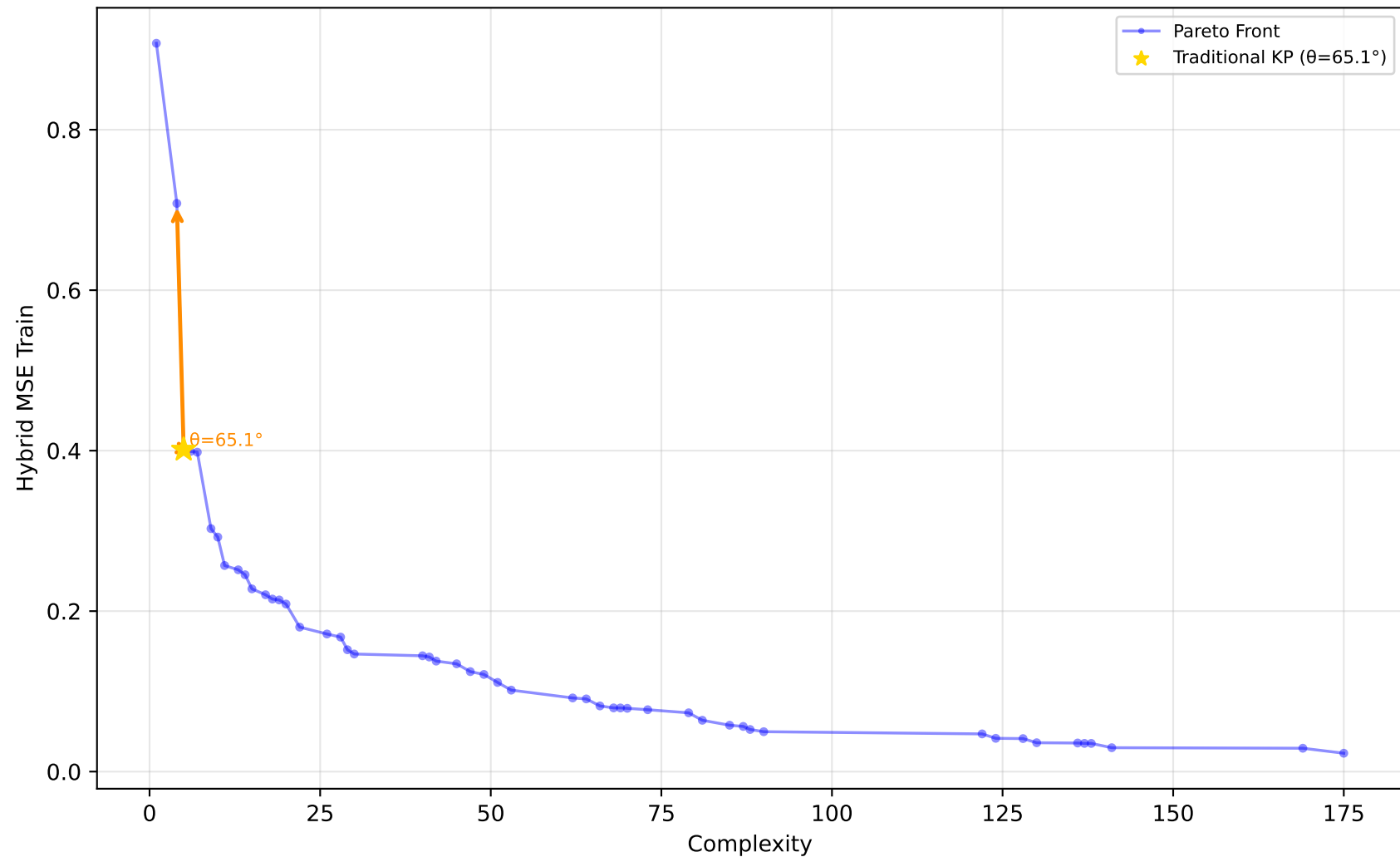
1028_SWD - Run 19 - SVP - Hybrid MSE Train \lambda_1=0.00, \lambda_2=0.60, \lambda_3=0.00 | Difficulty: 1.00 | Method: hmr
