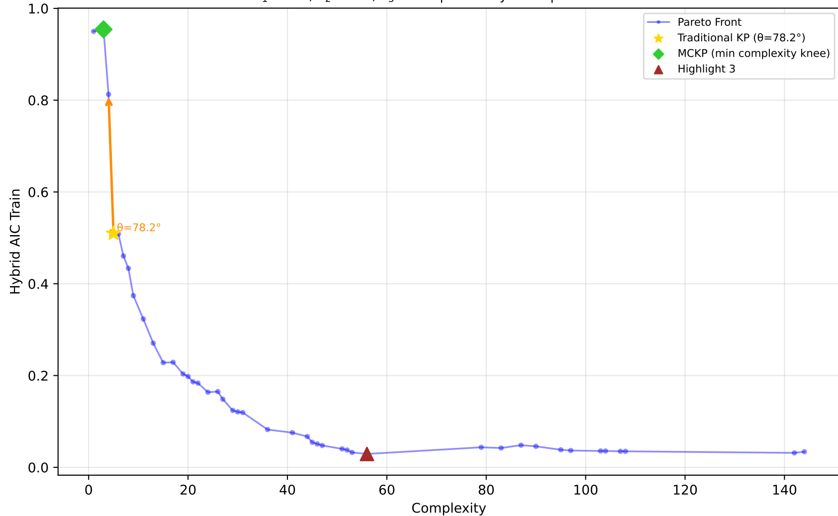
1028_SWD - Run 1 - MVP - Hybrid AIC Train \lambda_1=0.00, \lambda_2=0.00, \lambda_3=0.00 | Difficulty: 1.00 | Method: hmr
