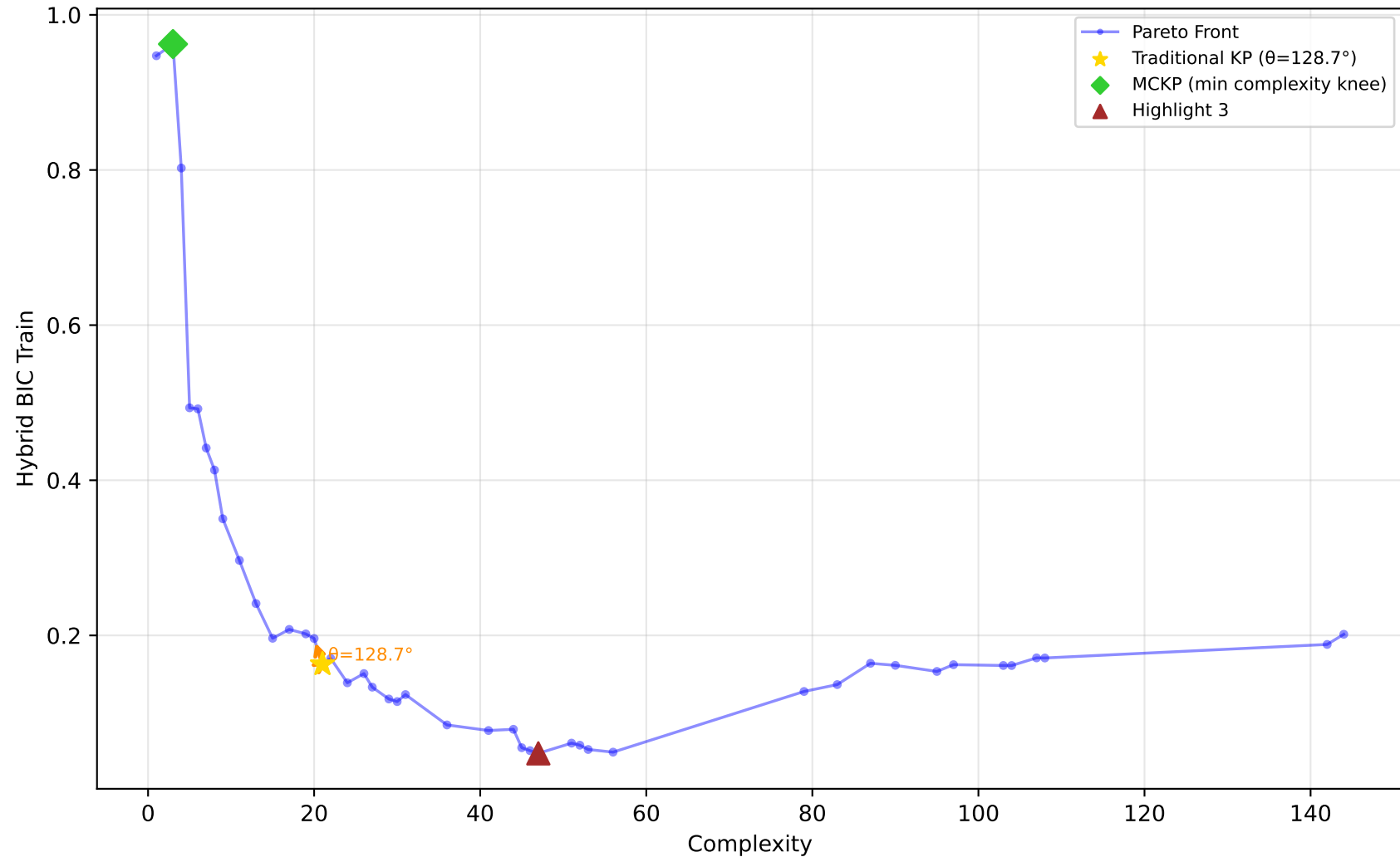
1028_SWD - Run 1 - MVP - Hybrid BIC Train \lambda_1=0.00, \lambda_2=0.00, \lambda_3=0.00 | Difficulty: 1.00 | Method: hmr
