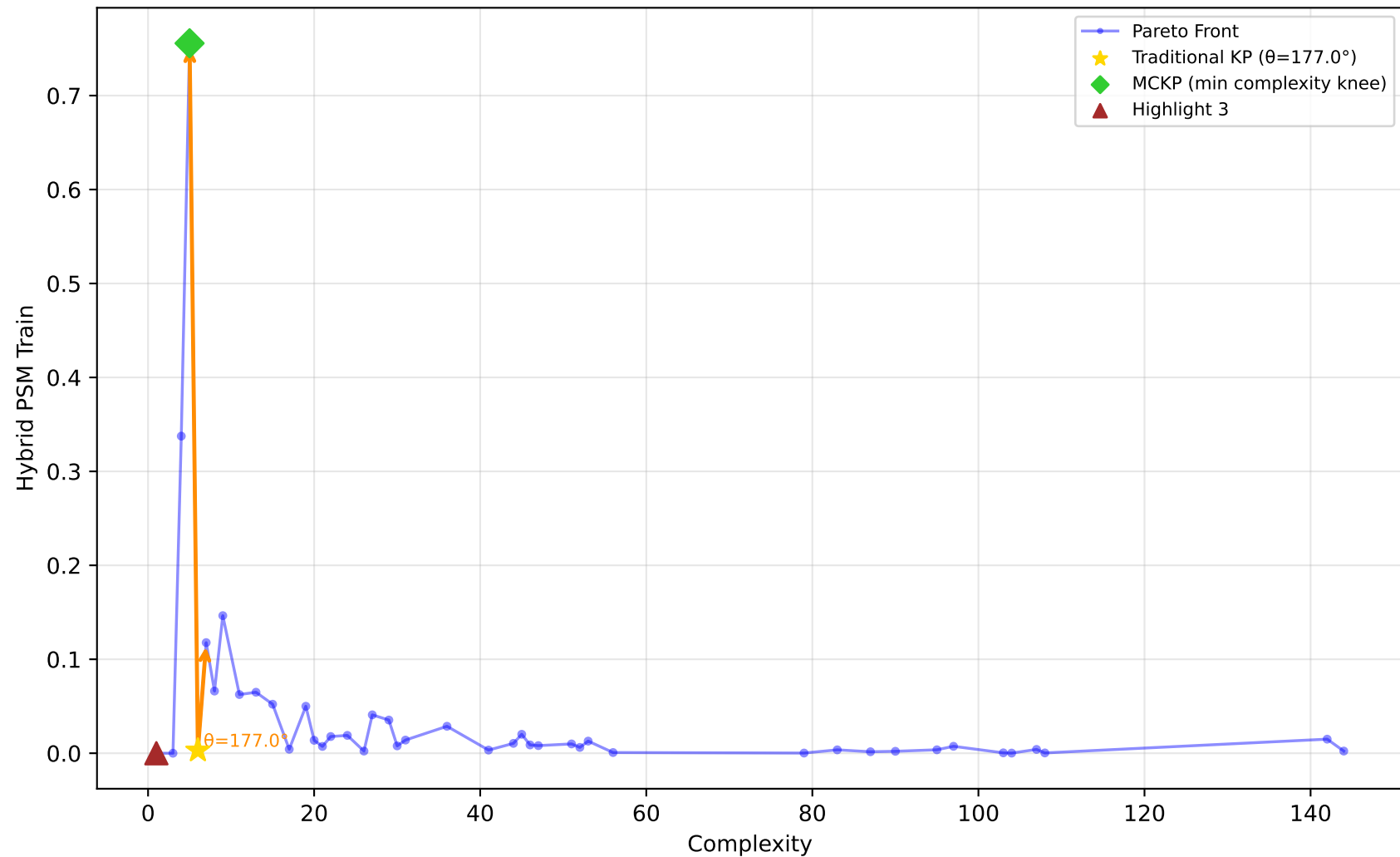
1028_SWD - Run 1 - MVP - Hybrid PSM Train \lambda_1=0.00, \lambda_2=0.00, \lambda_3=0.00 | Difficulty: 1.00 | Method: hmr
