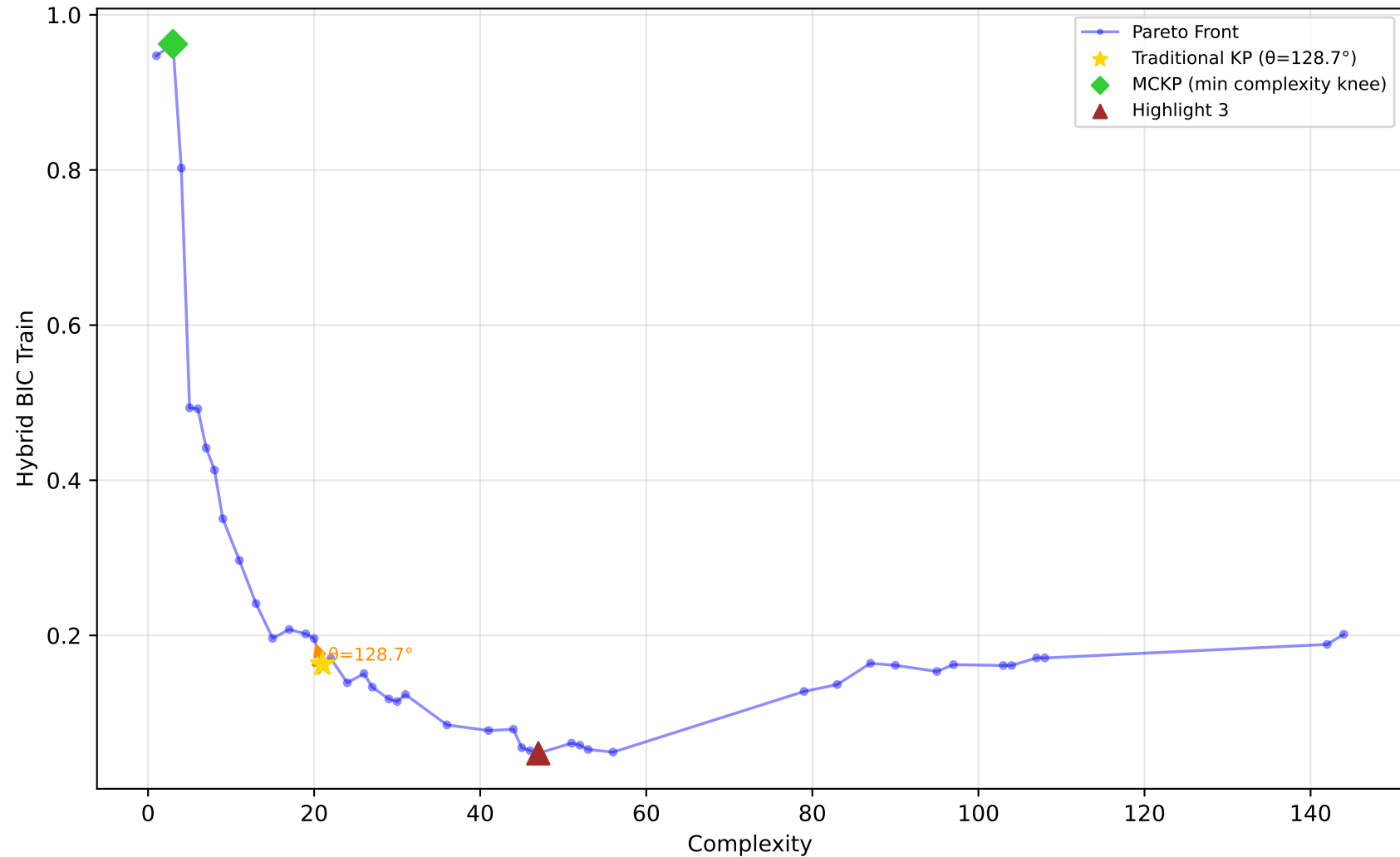
1028_SWD - Run 1 - SVP - Hybrid BIC Train \lambda_1=0.00, \lambda_2=0.60, \lambda_3=0.00 | Difficulty: 1.00 | Method: hmr
