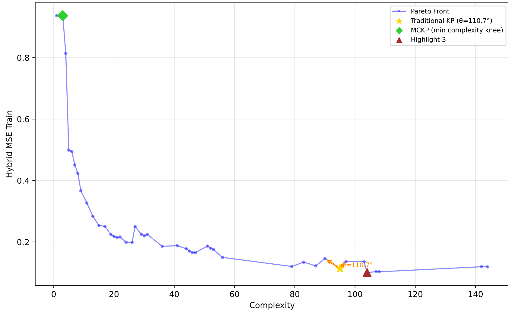
1028_SWD - Run 1 - SVP - Hybrid MSE Train \lambda_1=0.60, \lambda_2=0.00, \lambda_3=0.00 | Difficulty: 1.00 | Method: hmr
