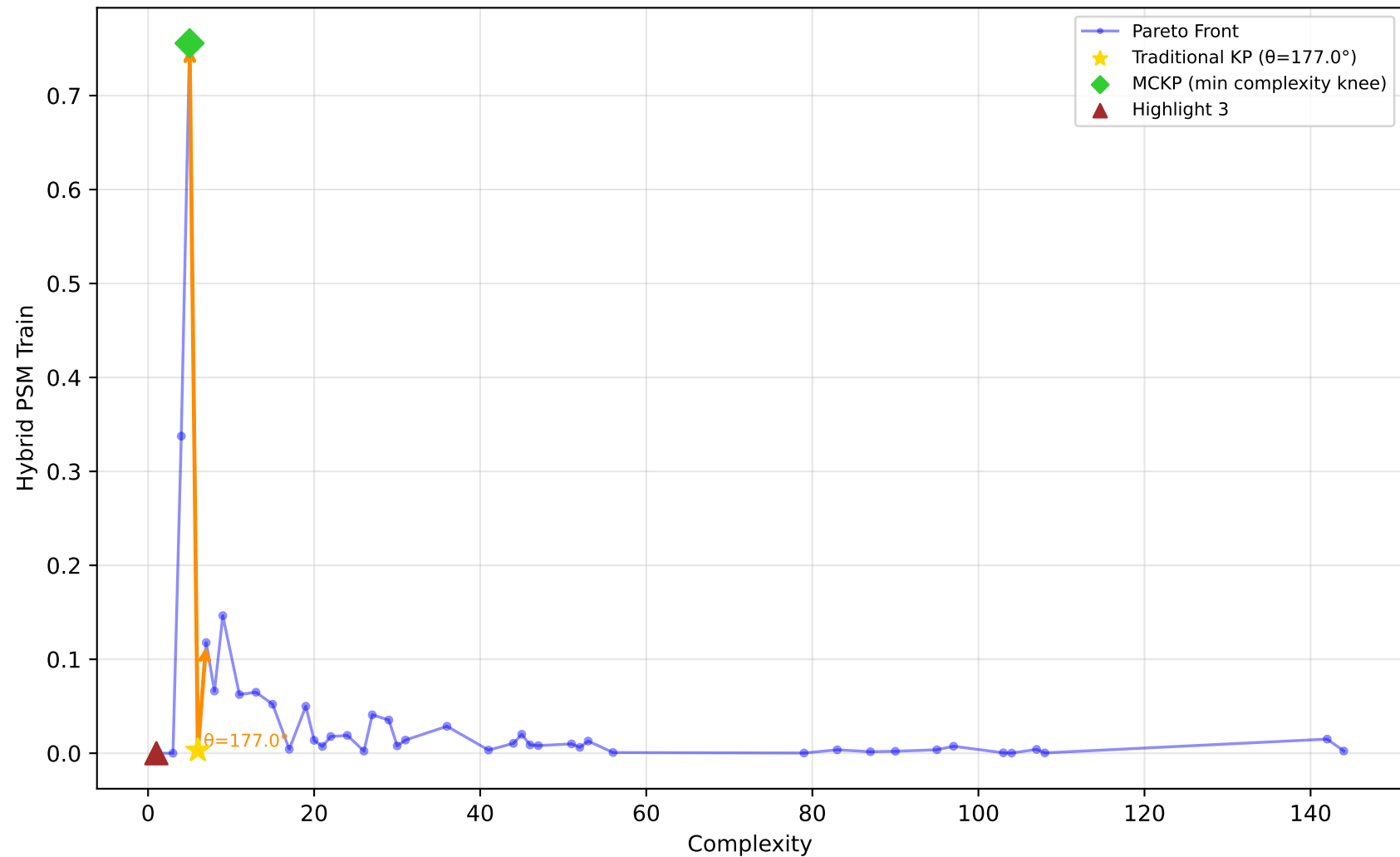
1028_SWD - Run 1 - SVP - Hybrid PSM Train \lambda_1=0.00, \lambda_2=0.60, \lambda_3=0.00 | Difficulty: 1.00 | Method: hmr
