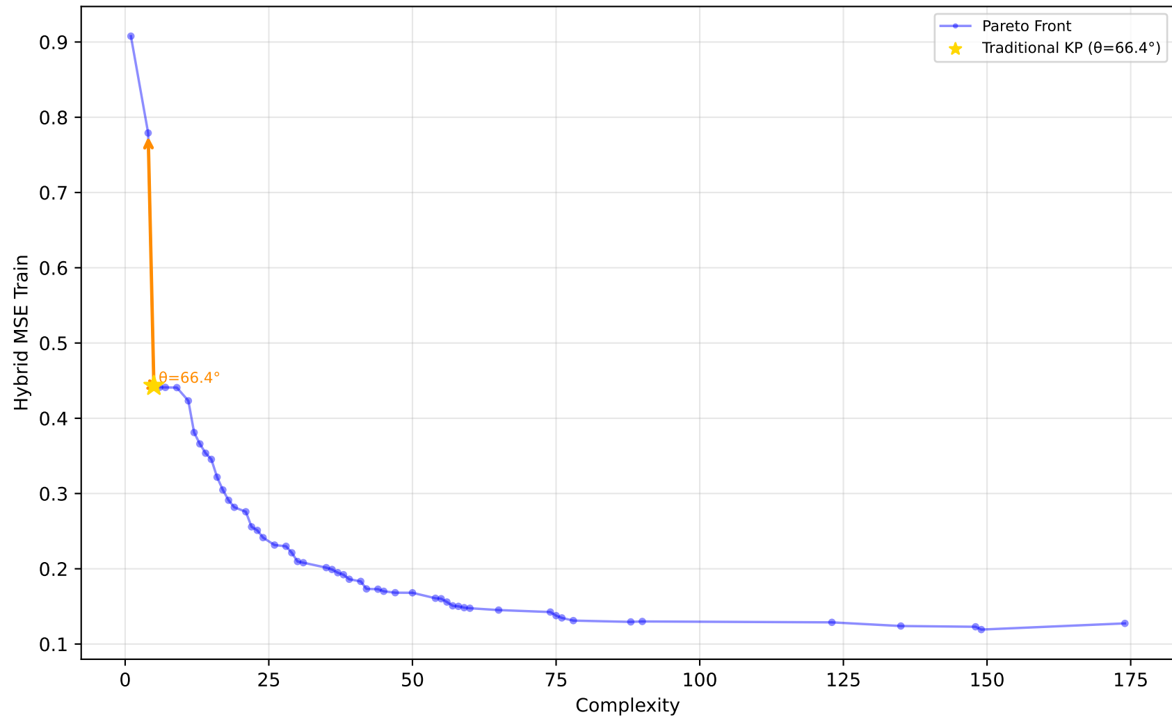
1028_SWD - Run 20 - MVP - Hybrid MSE Train \lambda_1=0.00, \lambda_2=0.00, \lambda_3=0.00 | Difficulty: 1.00 | Method: hmr
