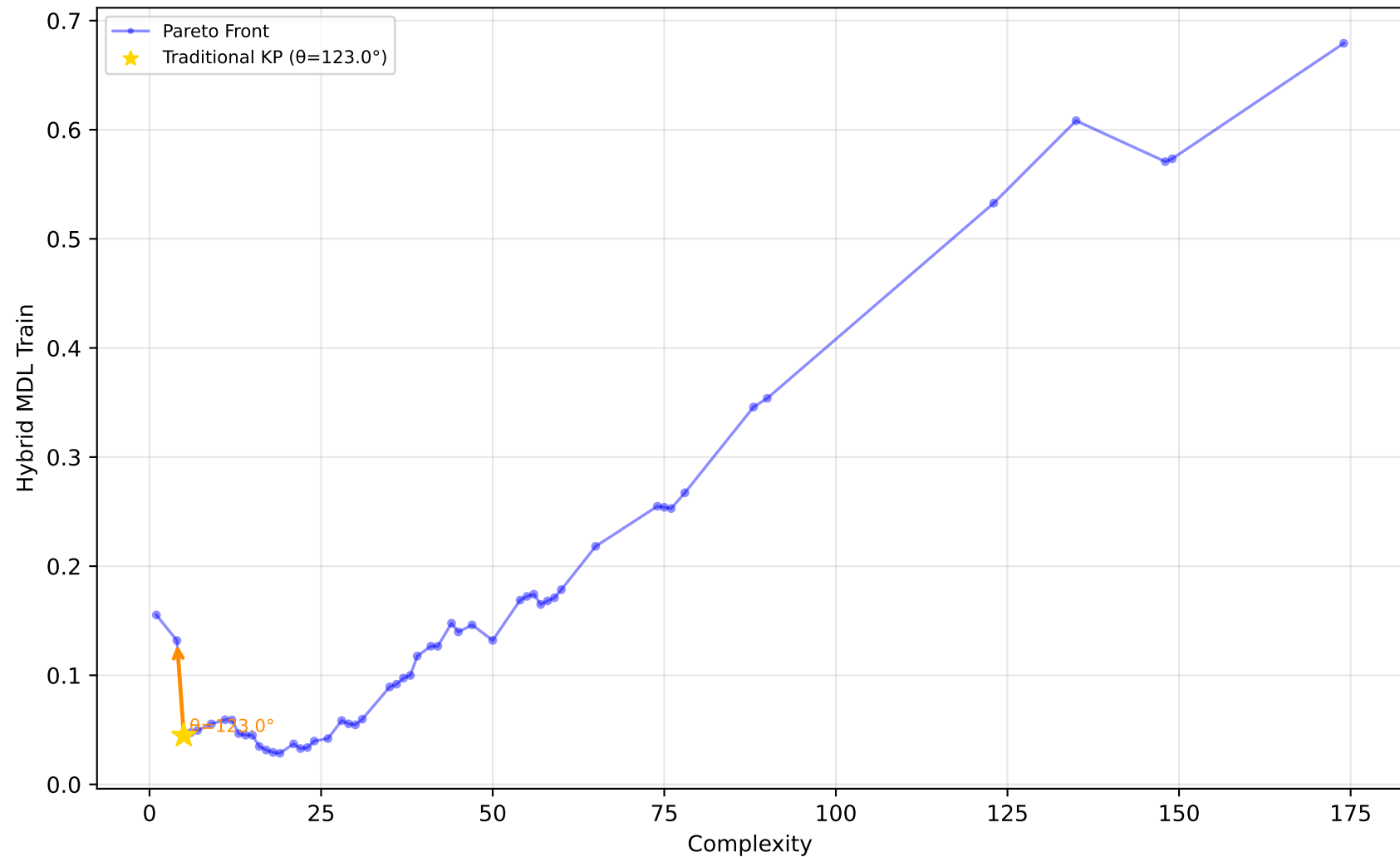
1028_SWD - Run 20 - SVP - Hybrid MDL Train \lambda_1=0.00, \lambda_2=0.60, \lambda_3=0.00 | Difficulty: 1.00 | Method: hmr
