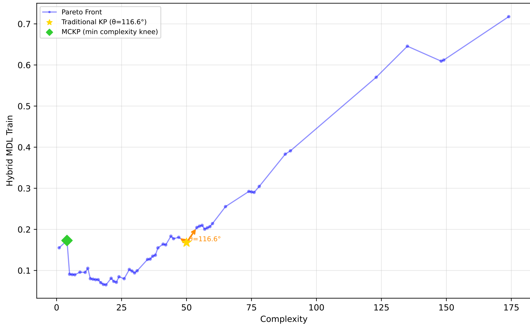
1028_SWD - Run 20 - SVP - Hybrid MDL Train \lambda_1=0.60, \lambda_2=0.00, \lambda_3=0.00 | Difficulty: 1.00 | Method: hmr
