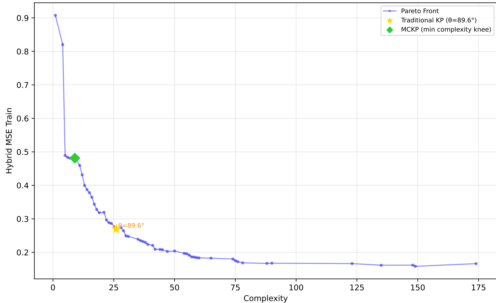
1028_SWD - Run 20 - SVP - Hybrid MSE Train \lambda_1=0.60, \lambda_2=0.00, \lambda_3=0.00 | Difficulty: 1.00 | Method: hmr
