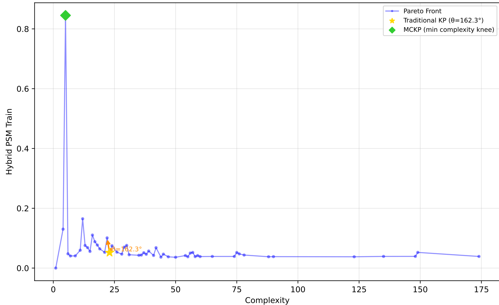
1028_SWD - Run 20 - SVP - Hybrid PSM Train \lambda_1=0.60, \lambda_2=0.00, \lambda_3=0.00 | Difficulty: 1.00 | Method: hmr
