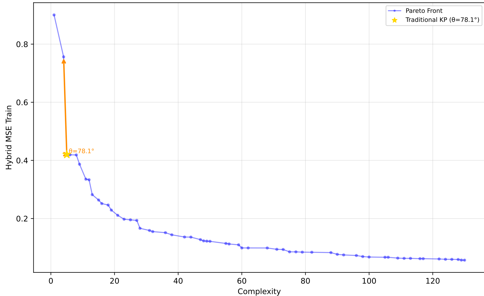
1028_SWD - Run 21 - MVP - Hybrid MSE Train \lambda_1=0.00, \lambda_2=0.00, \lambda_3=0.00 | Difficulty: 1.00 | Method: hmr
