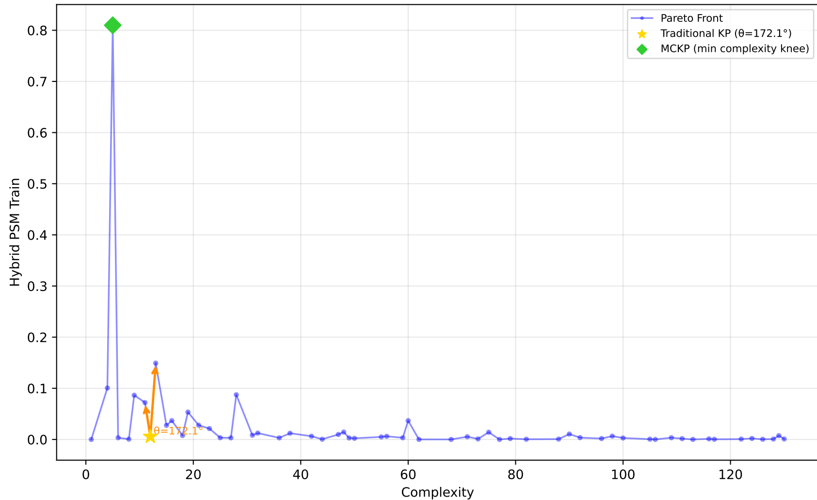
1028_SWD - Run 21 - MVP - Hybrid PSM Train \lambda_1=0.00, \lambda_2=0.00, \lambda_3=0.00 | Difficulty: 1.00 | Method: hmr
