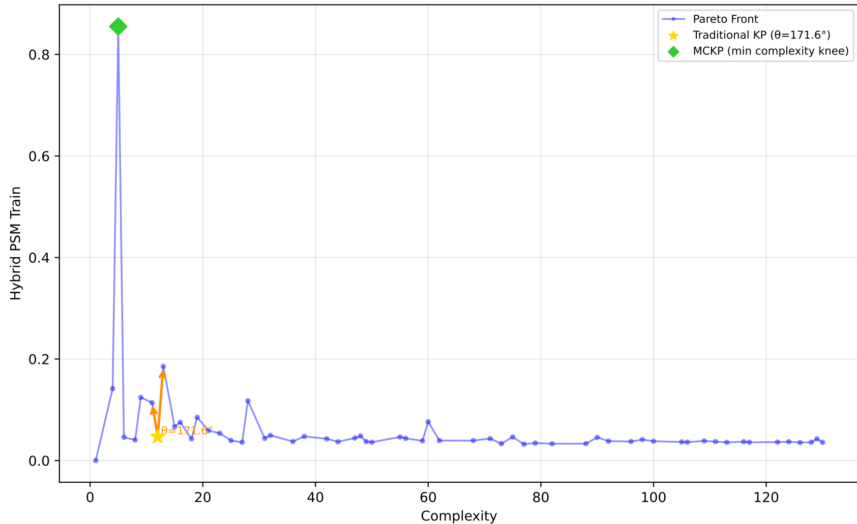
1028_SWD - Run 21 - MVP - Hybrid PSM Train \lambda_1=0.60, \lambda_2=0.00, \lambda_3=0.00 | Difficulty: 1.00 | Method: hmr
