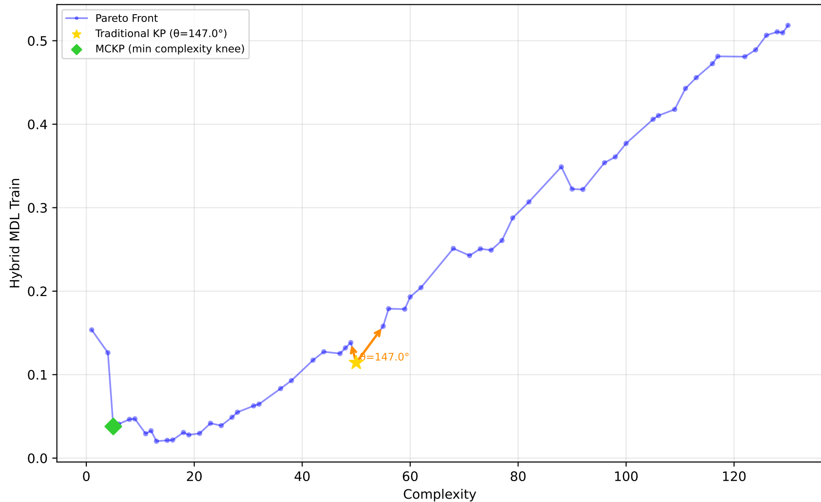
1028_SWD - Run 21 - SVP - Hybrid MDL Train \lambda_1=0.00, \lambda_2=0.60, \lambda_3=0.00 | Difficulty: 1.00 | Method: hmr
