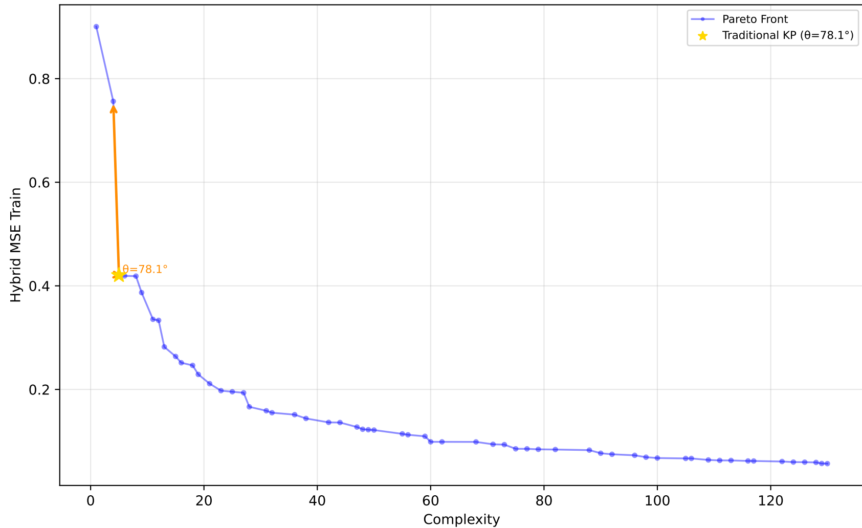
1028_SWD - Run 21 - SVP - Hybrid MSE Train \lambda_1=0.00, \lambda_2=0.60, \lambda_3=0.00 | Difficulty: 1.00 | Method: hmr
