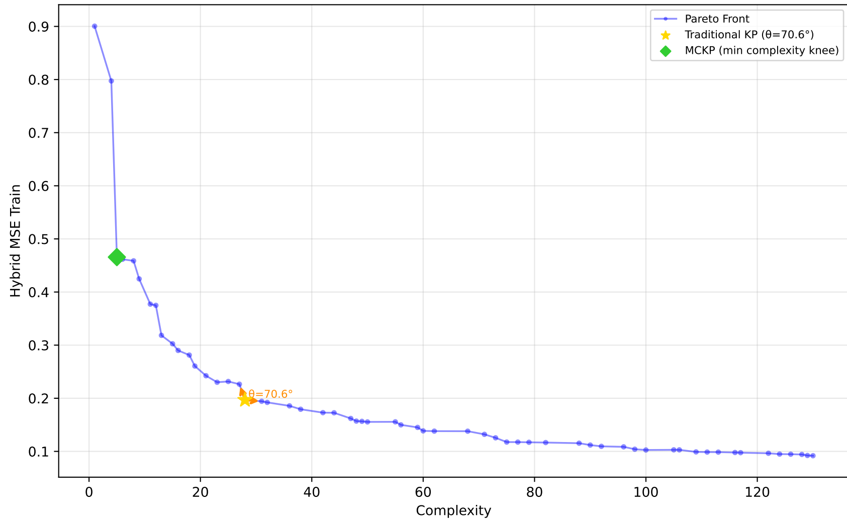
1028_SWD - Run 21 - SVP - Hybrid MSE Train \lambda_1=0.60, \lambda_2=0.00, \lambda_3=0.00 | Difficulty: 1.00 | Method: hmr
