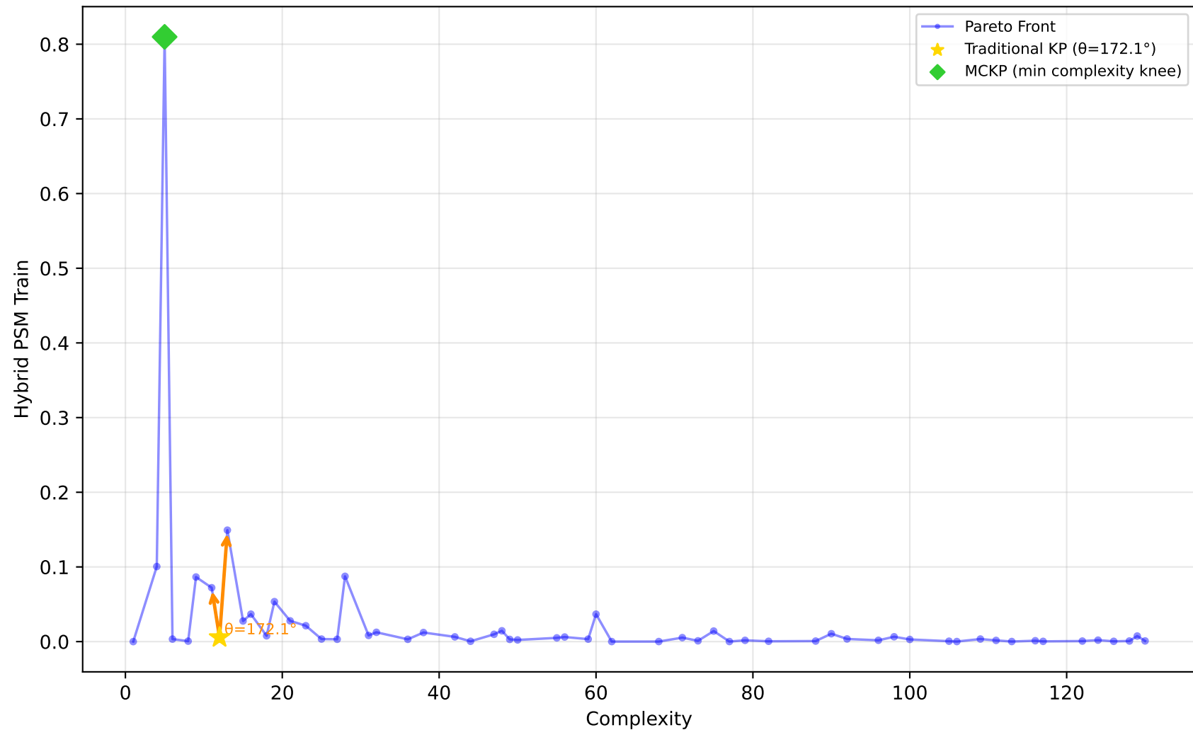
1028_SWD - Run 21 - SVP - Hybrid PSM Train \lambda_1=0.00, \lambda_2=0.60, \lambda_3=0.00 | Difficulty: 1.00 | Method: hmr
