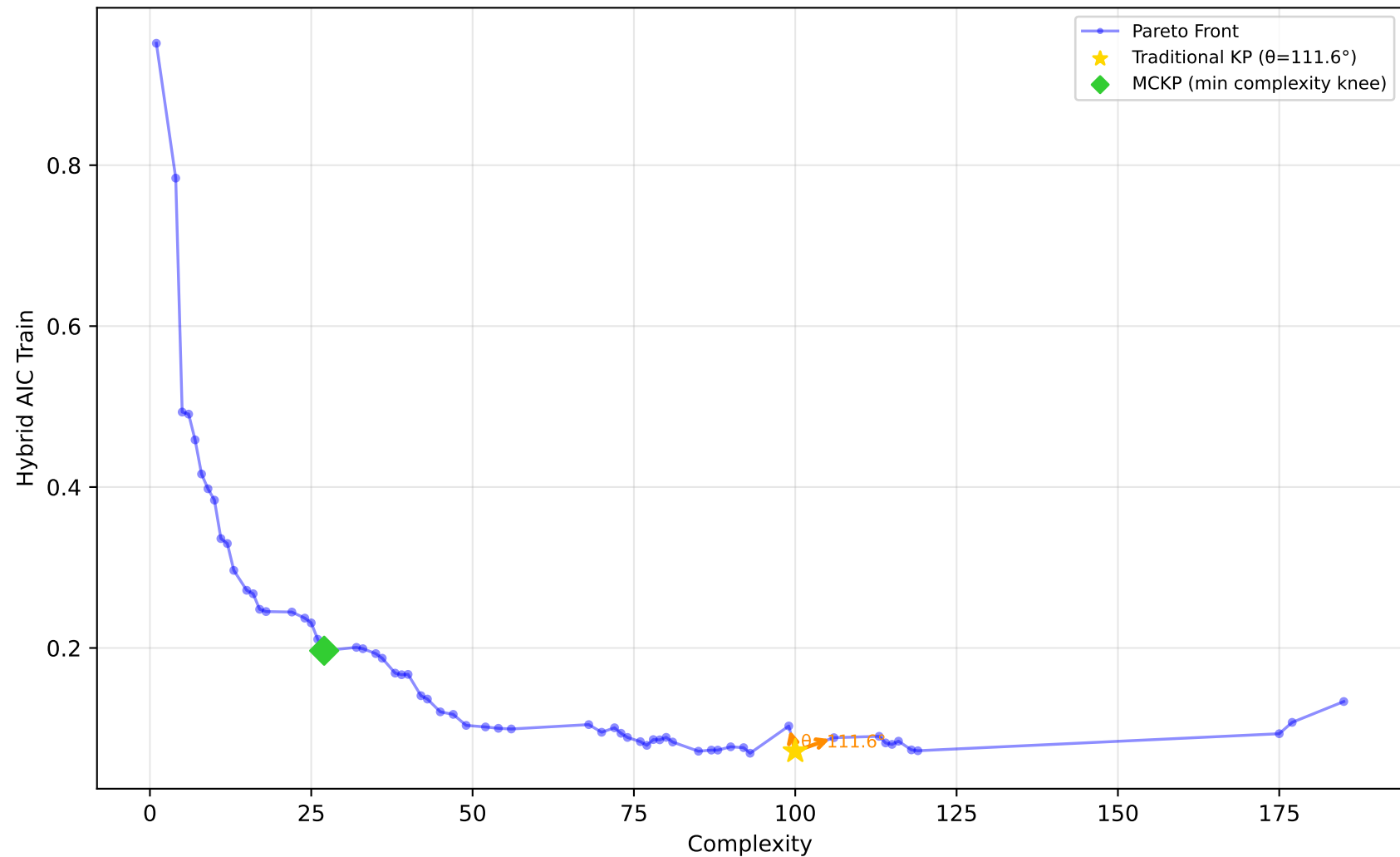
1028_SWD - Run 22 - MVP - Hybrid AIC Train \lambda_1=0.00, \lambda_2=0.00, \lambda_3=0.00 | Difficulty: 1.00 | Method: hmr
