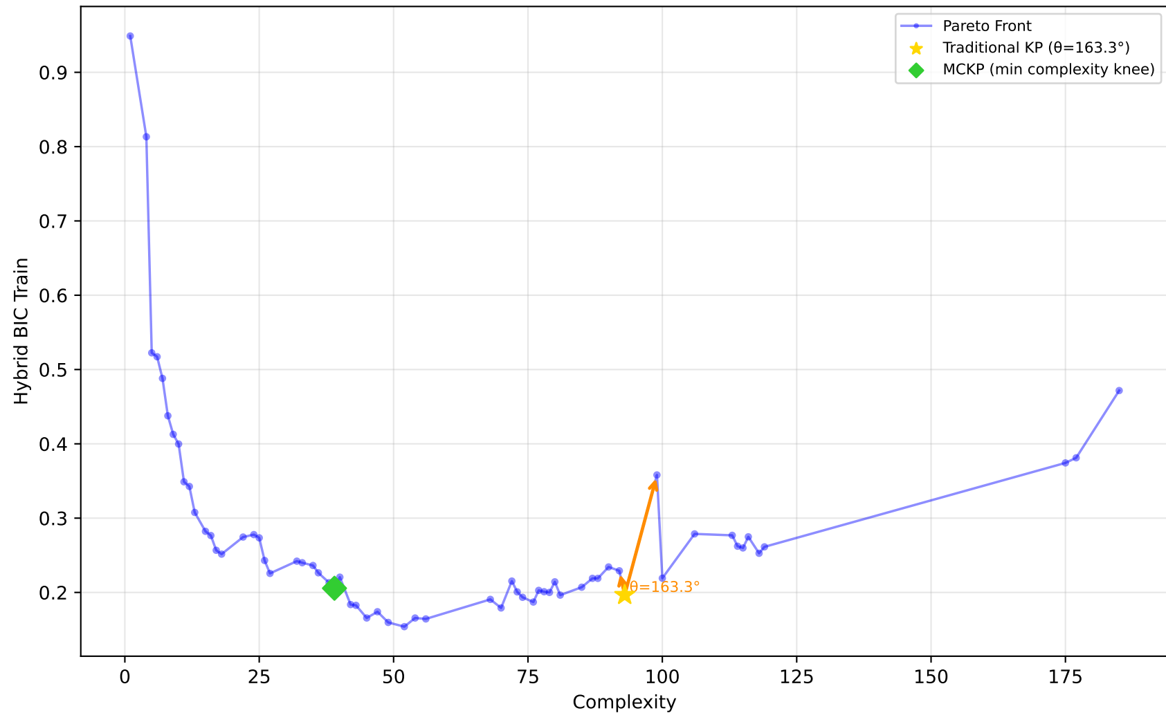
1028_SWD - Run 22 - MVP - Hybrid BIC Train \lambda_1=0.60, \lambda_2=0.00, \lambda_3=0.00 | Difficulty: 1.00 | Method: hmr
