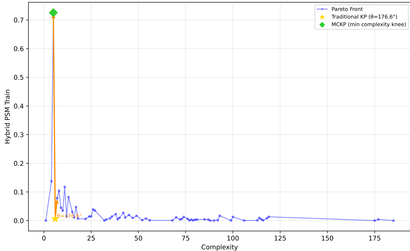
1028_SWD - Run 22 - MVP - Hybrid PSM Train \lambda_1=0.00, \lambda_2=0.00, \lambda_3=0.00 | Difficulty: 1.00 | Method: hmr
