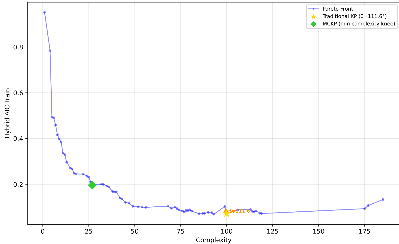
1028_SWD - Run 22 - SVP - Hybrid AIC Train \lambda_1=0.00, \lambda_2=0.60, \lambda_3=0.00 | Difficulty: 1.00 | Method: hmr
